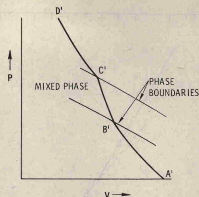
FIG. 32. Projection of phase boundaries and R-H curves of Fig. 31 onto the pressure-volume plane.
