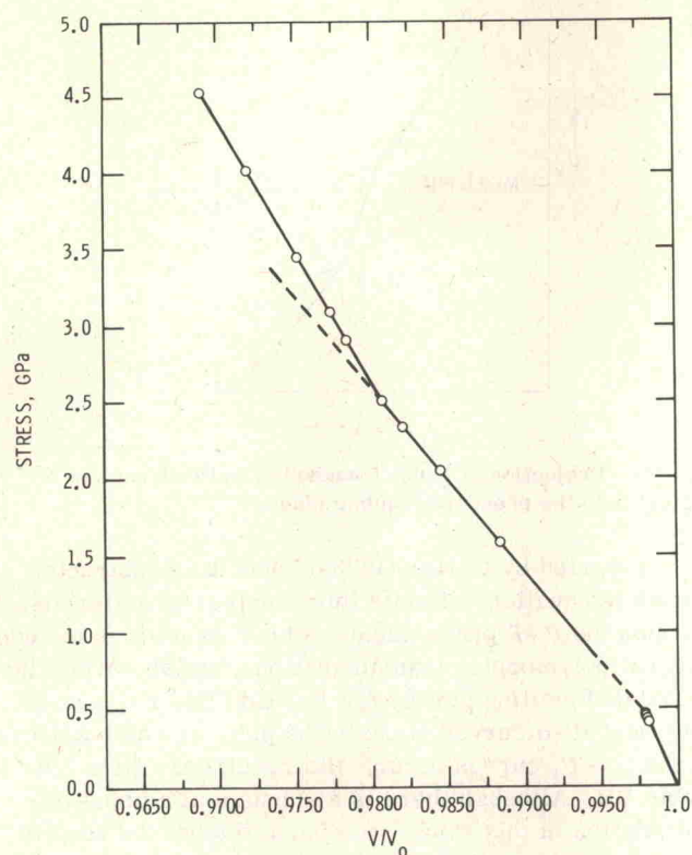
FIG. 30. The stress versus volume relation for a low carbon 28.4 at. % Ni-Fe alloy in the fcc phase shows a second-order phase transition indicated by a large decrease in compressibility at stress of 2.50 GPa. The dashed line indicates an extension of the compressibility of the lower stress data. When a correction for shear strength is applied to the shock data to account for the 0.45 GPa Hugoniot elastic limit, excellent agreement is noted between shock and static loading determinations of the dependence of Curie temperature on pressure. After Graham et al. (1967).
