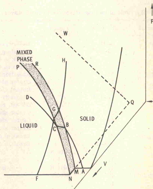
FIG. 31. P - V - T surface for a normal liquid and solid. The mixed phase region is bounded by RPNM .
